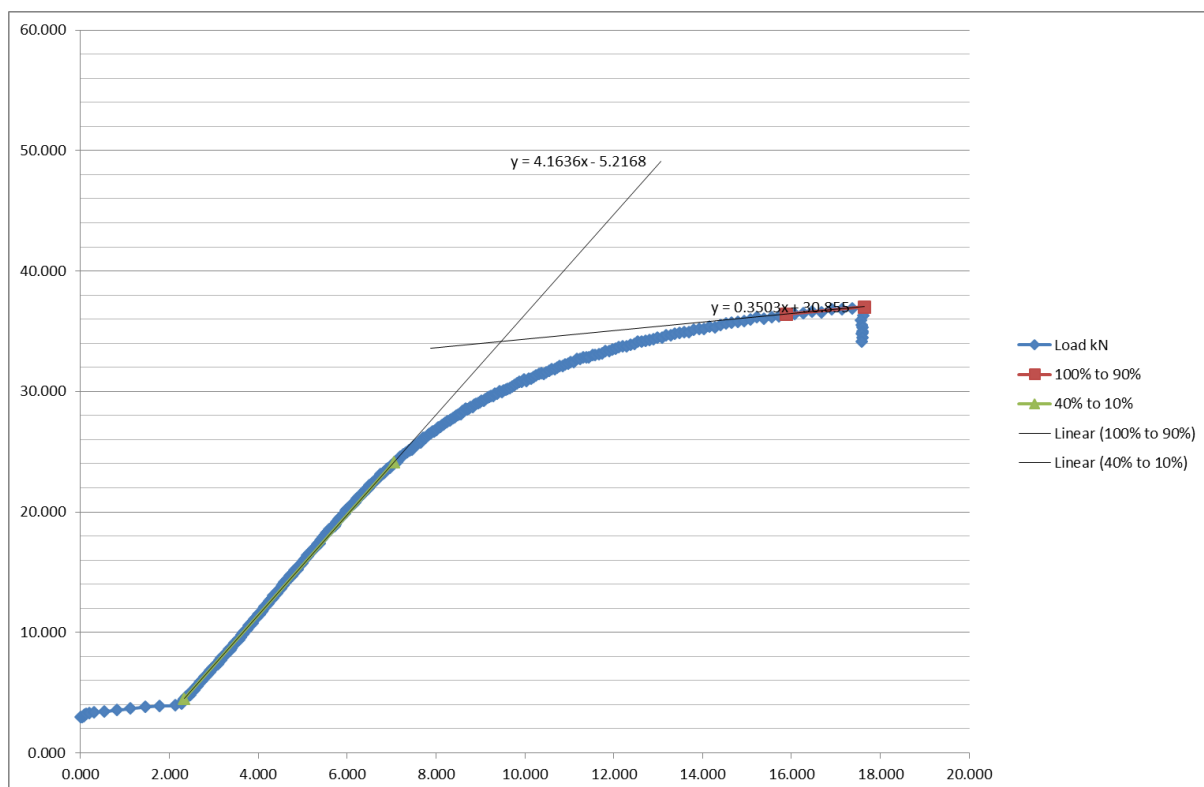
Figure G.I Example estimation of yield strength
