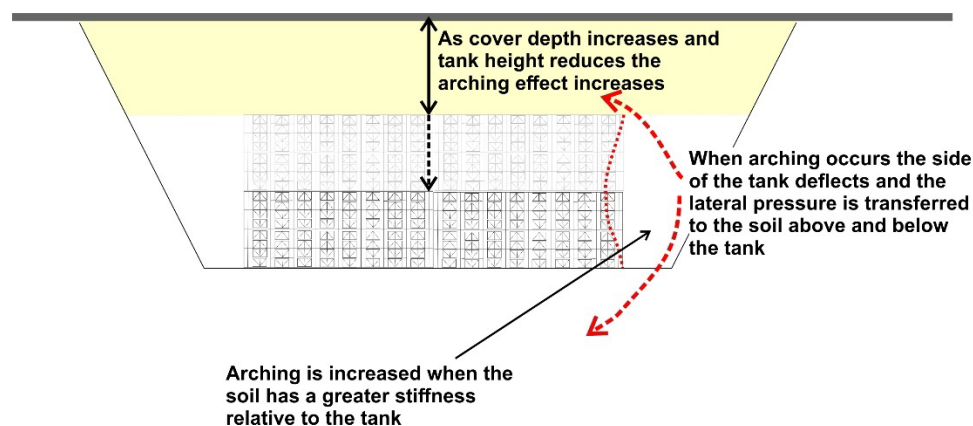
Figure 5 Arching around a geocellular tank
