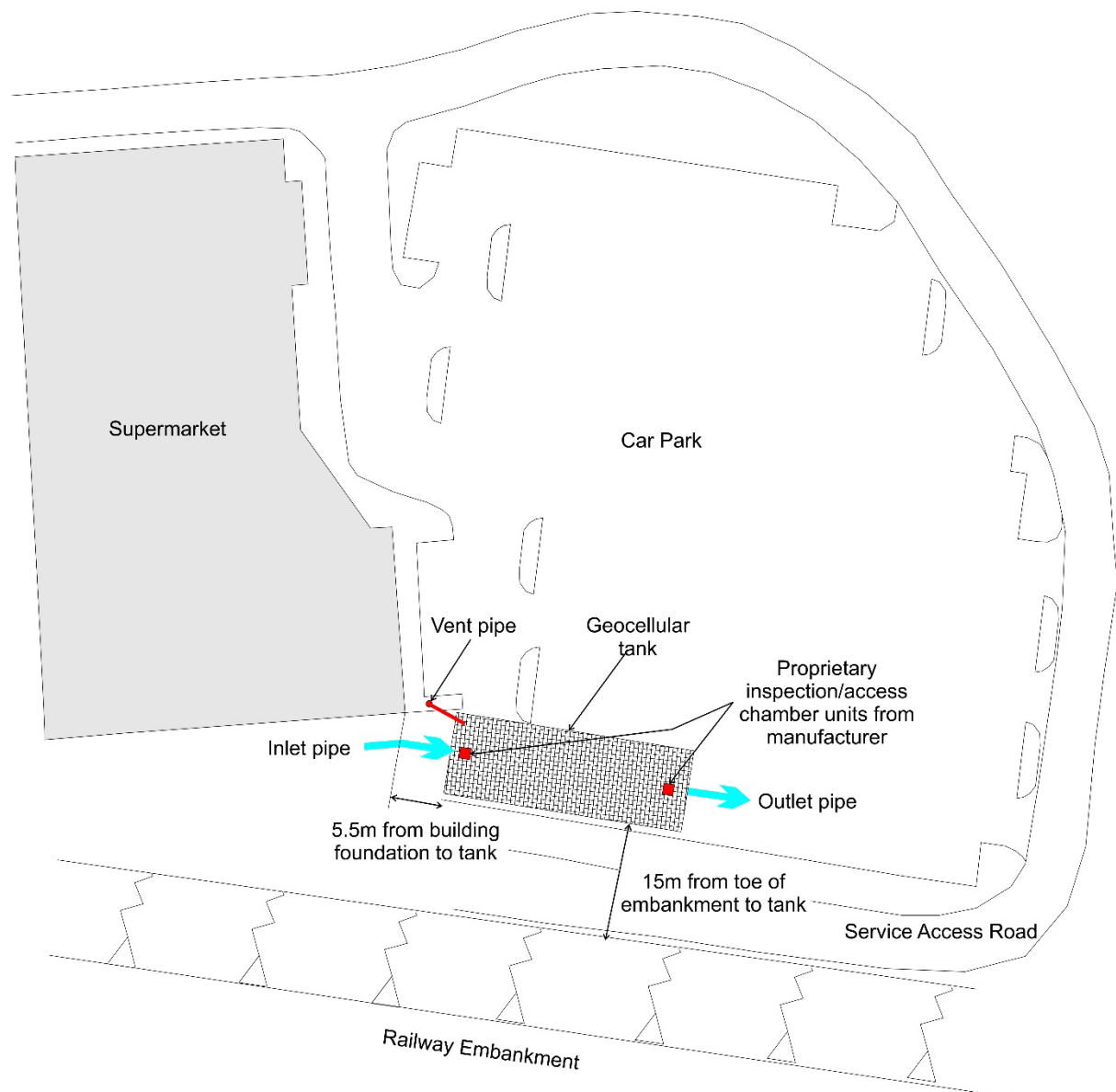
Figure 1 Example scheme general arrangement
