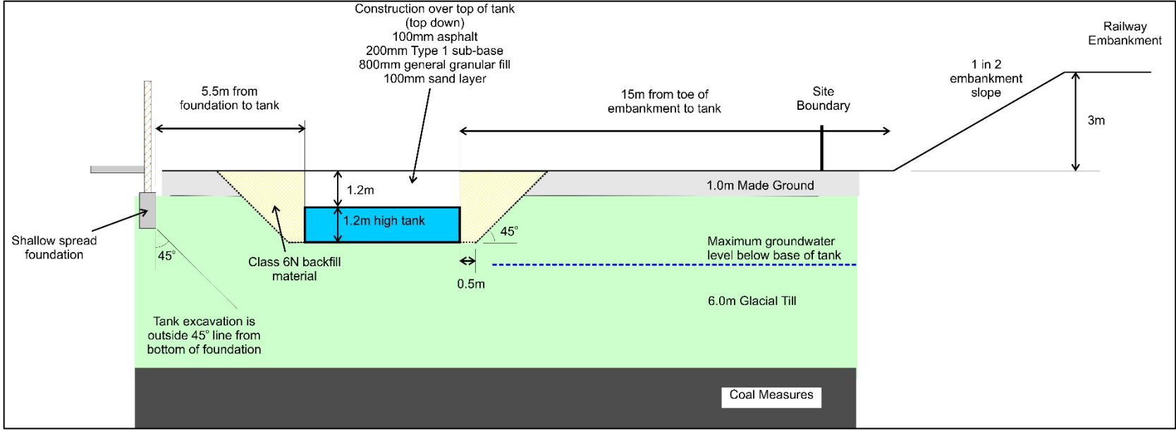
Figure 2 Example conceptual ground model
