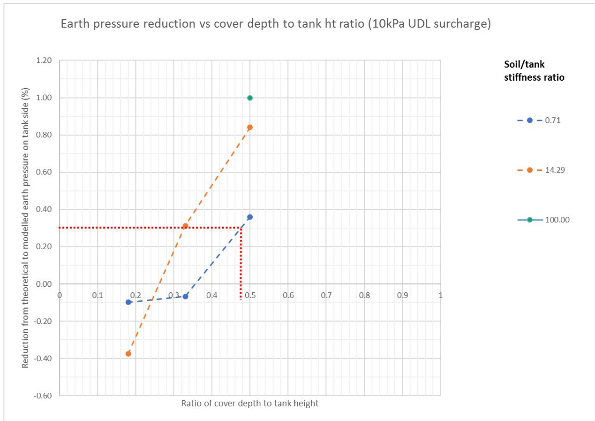
Figure E.3 Earth pressure reduction against ratio of cover depth to tank height for surcharge
