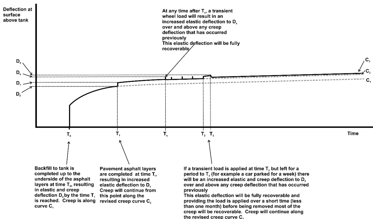
Figure 6 Deflection at ground surface during and after construction
