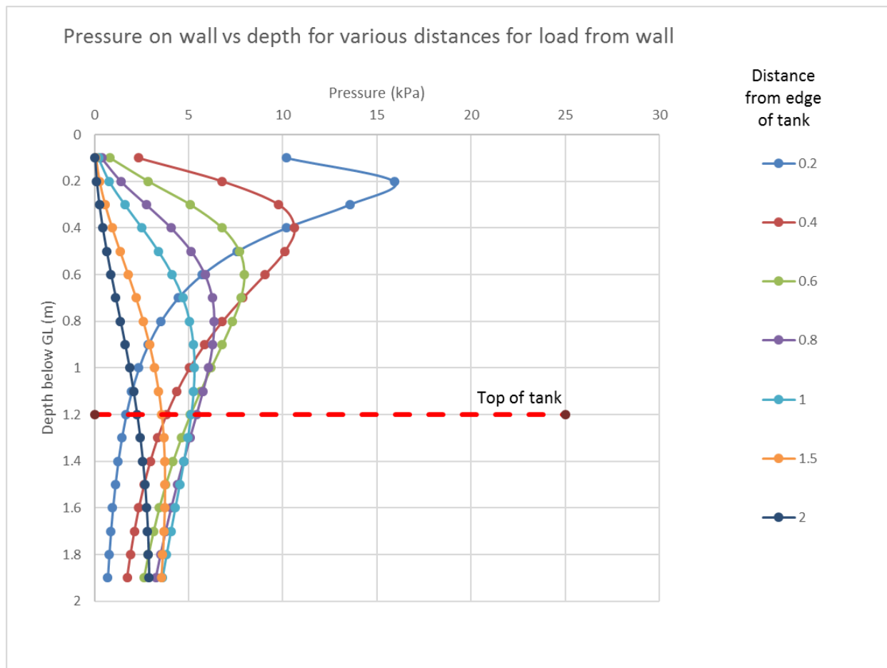
Figure 4 Variation of pressure on side of tank from wheel load for this example
