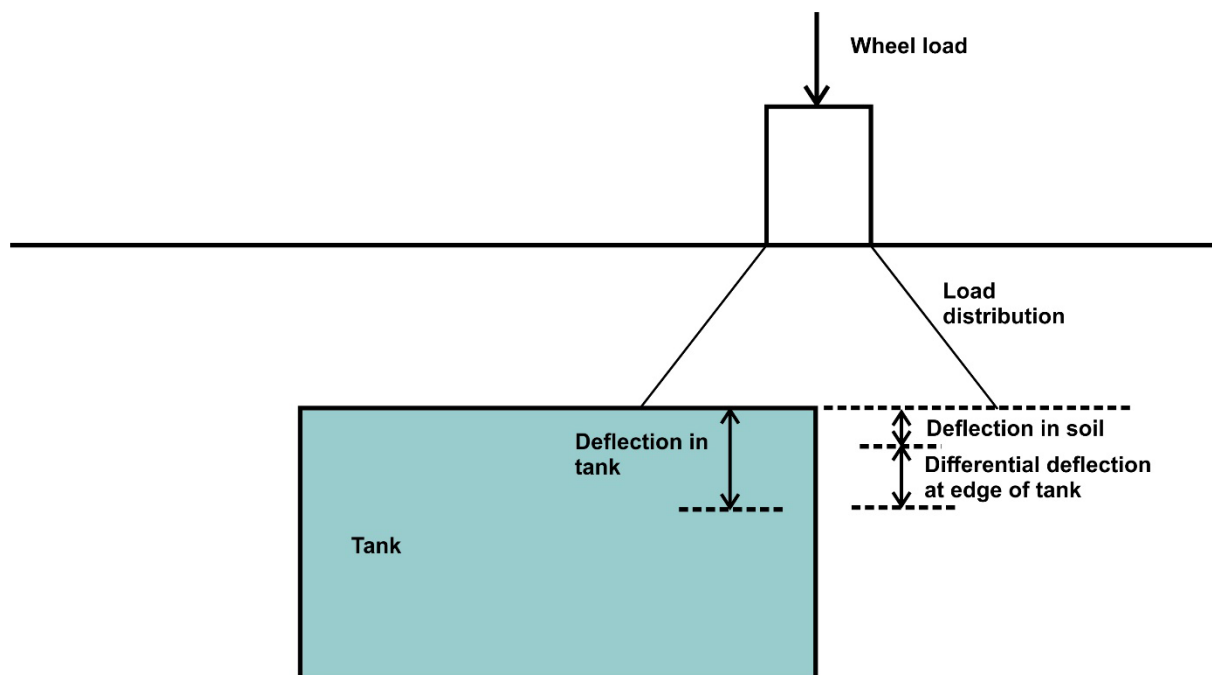
Figure 7 Tank deflection relative to surrounding area
