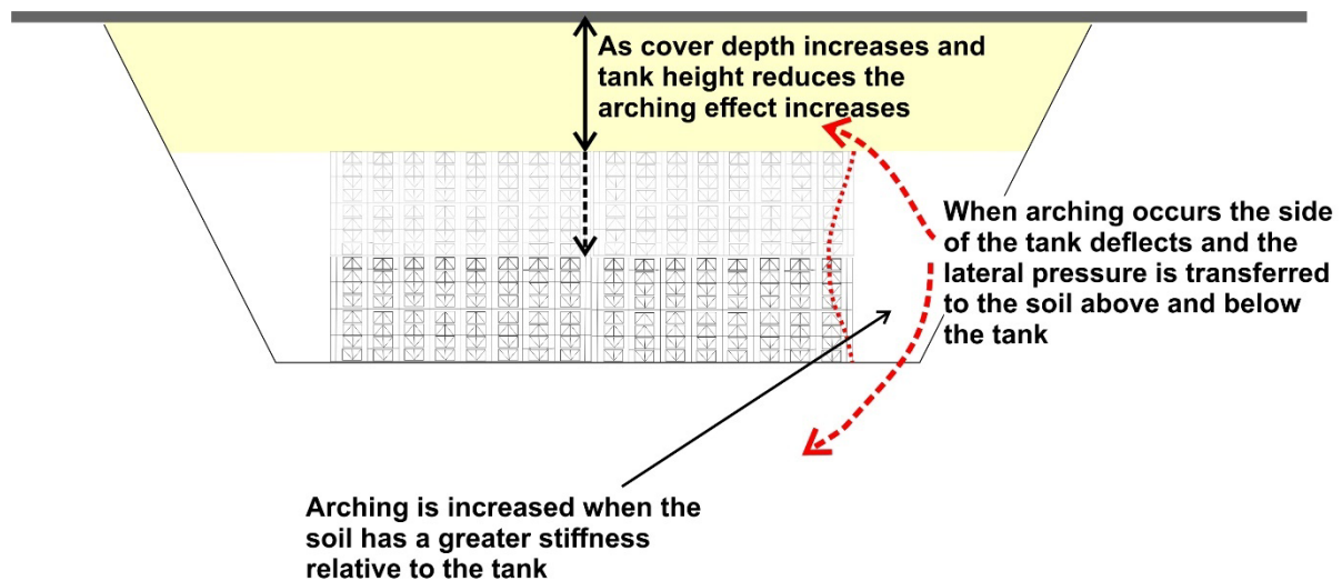
Figure E.1 Arching around a geocellular tank
