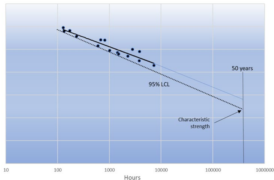
Figure 1 Regression analysis showing characteristic strength at 50 years
