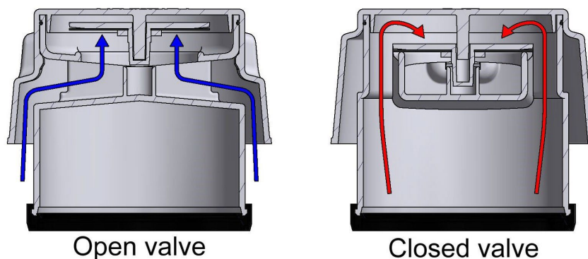
Figure 2 AAV operation
