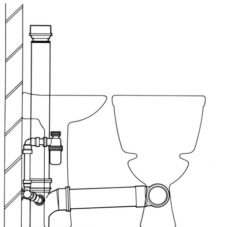
Figure 9 Installation of an AAV on a sub stack
