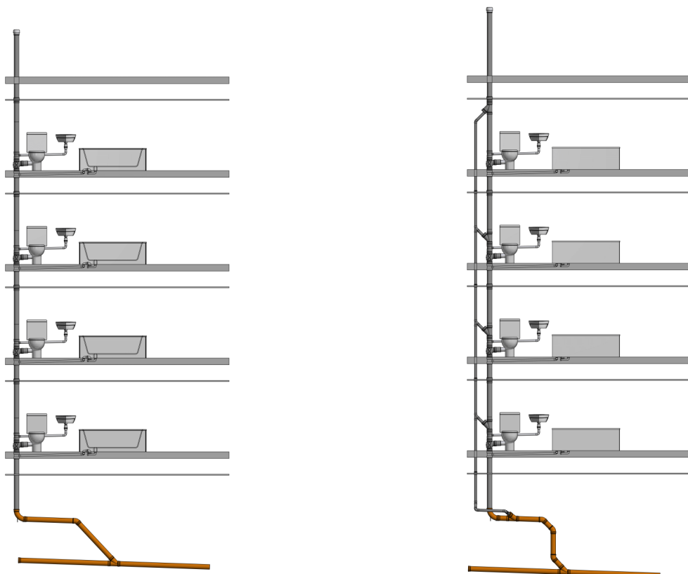
Figure 3 Stack ventilation options
